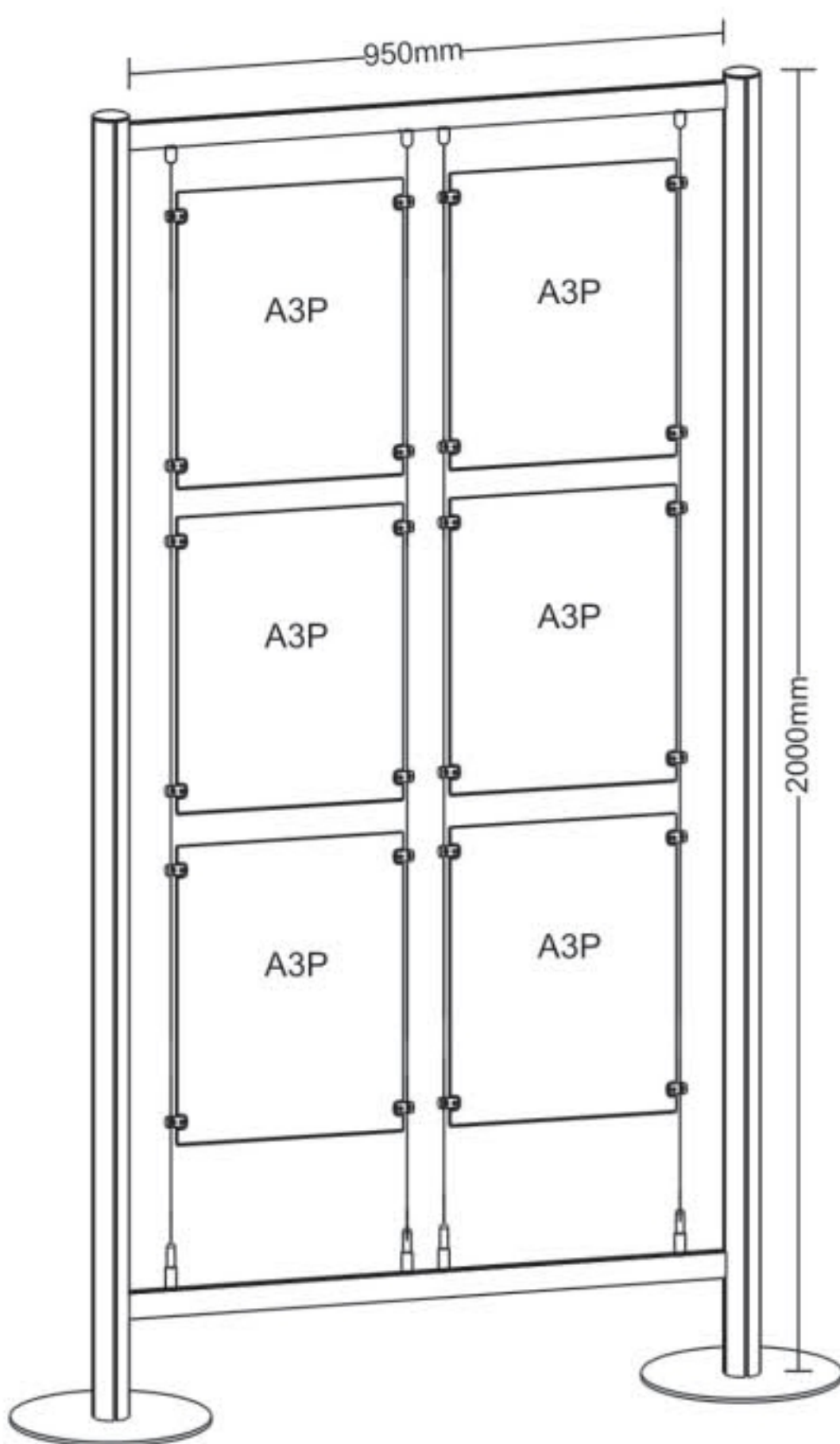
Free standing frames 6 A3 portrait 6 Double sided A3 Stand size : 950x2000mm Item No. 95020006
