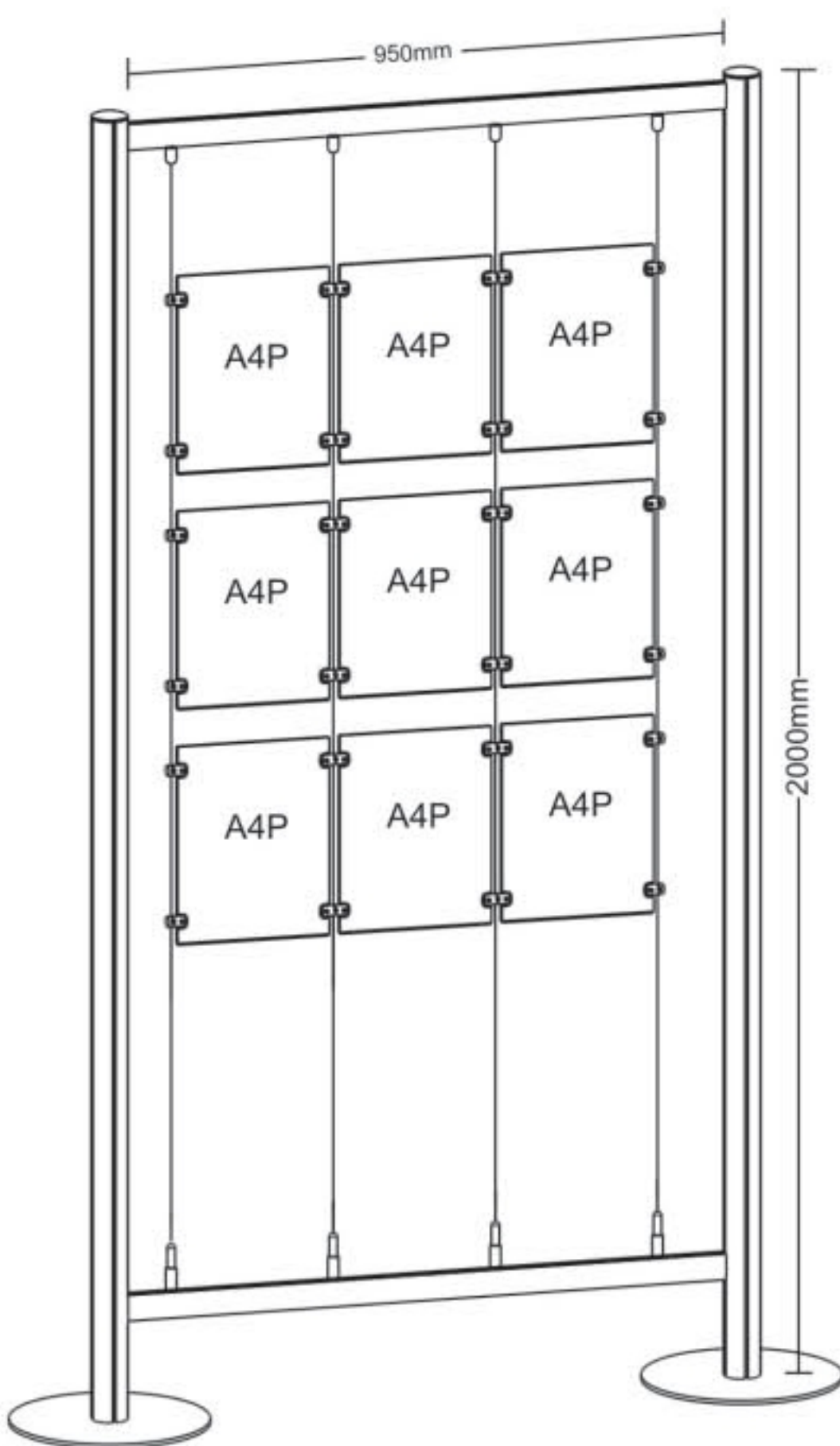
Free standing frames 9 A4 portrait 9 Double sided A4 Stand size : 950x2000mm Item No. 95020009
